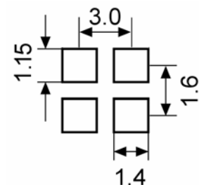
suggested soldering pad
