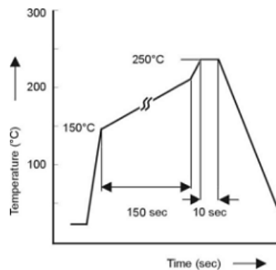
soldering condition
